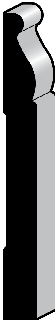
BASE P 813 9/16 x 5-1/4 PINE, FJPMD, FJPCC 1/2 x 5-1/4 MDF
