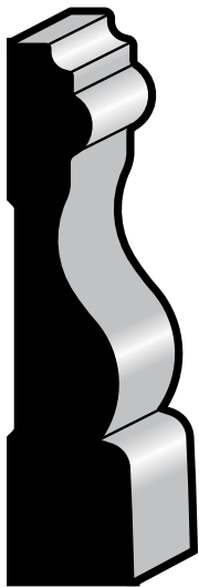
CASING 475 9/16 x 2-1/2 OAK
