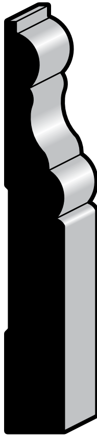
BASE POPFP 410 19/32 x 4-1/4
