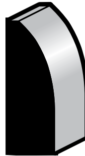
STOP 846 7/16 x 1-3/8 PINE, OAK
