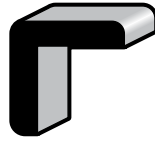
CORNER GUARD 205 1-1/16 x 1-1/16 OAK 206 3/4 x 3/4 OAK
