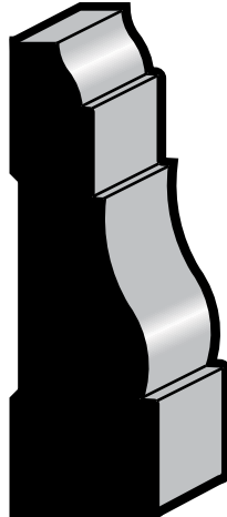
CASING 366 11/16 x 2-1/4 PINE, FJPM D, FJPCC 19/32 x 2-1/4 MDF 5/8 x 2-1/4 OAK, POPLR
