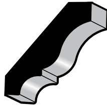
CROWN L 54 1/2 x 2-1/4 OAK
