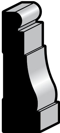
CASING 376 11/16 x 2-1/4 PINE, FJPM D 19/32 x 2-1/4 MDF
