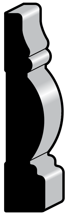
CASING 374 11/16 x 3-1/2 FJPCC, MDF, OAK 3/4 x 3-1/2
