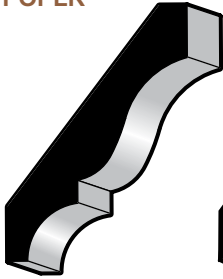
CROWN L 51 9/16 x 3-1/4 POPLR 1/2 x 3-1/4
