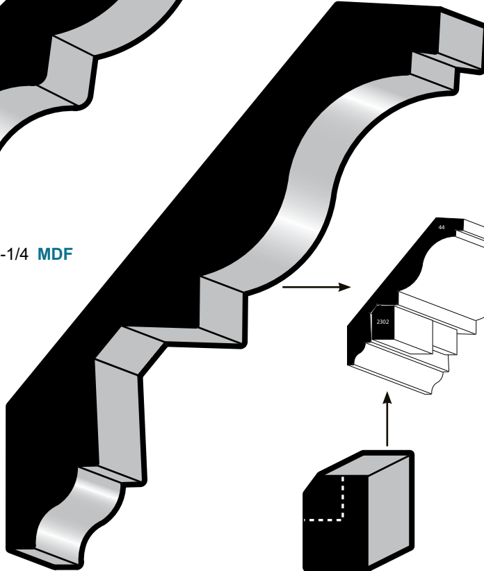
CROWN 45 13/16 x 5-1/4 OAK
