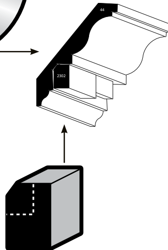
DENTIL MOULD 2302 11/16 x 15/16 OAK
