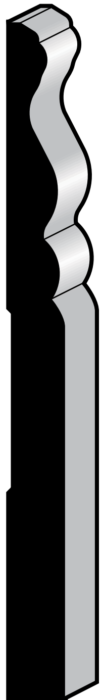
BASE 207 19/32 x 7-1/4 MDF
