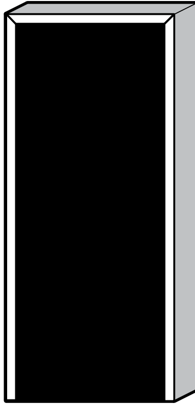
PLINTH BLOCK - BEVELED 916 27/32 x 2-1/2 x 5-3/4 OAK 917 1-1/8 x 3-1/2 x 6-1/2 PINE, OAK
