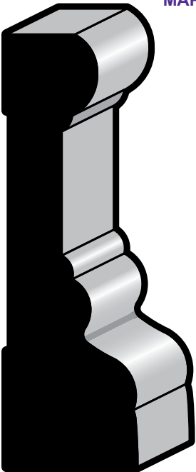
CASING PT3 1 x 3-1/4 MDF
