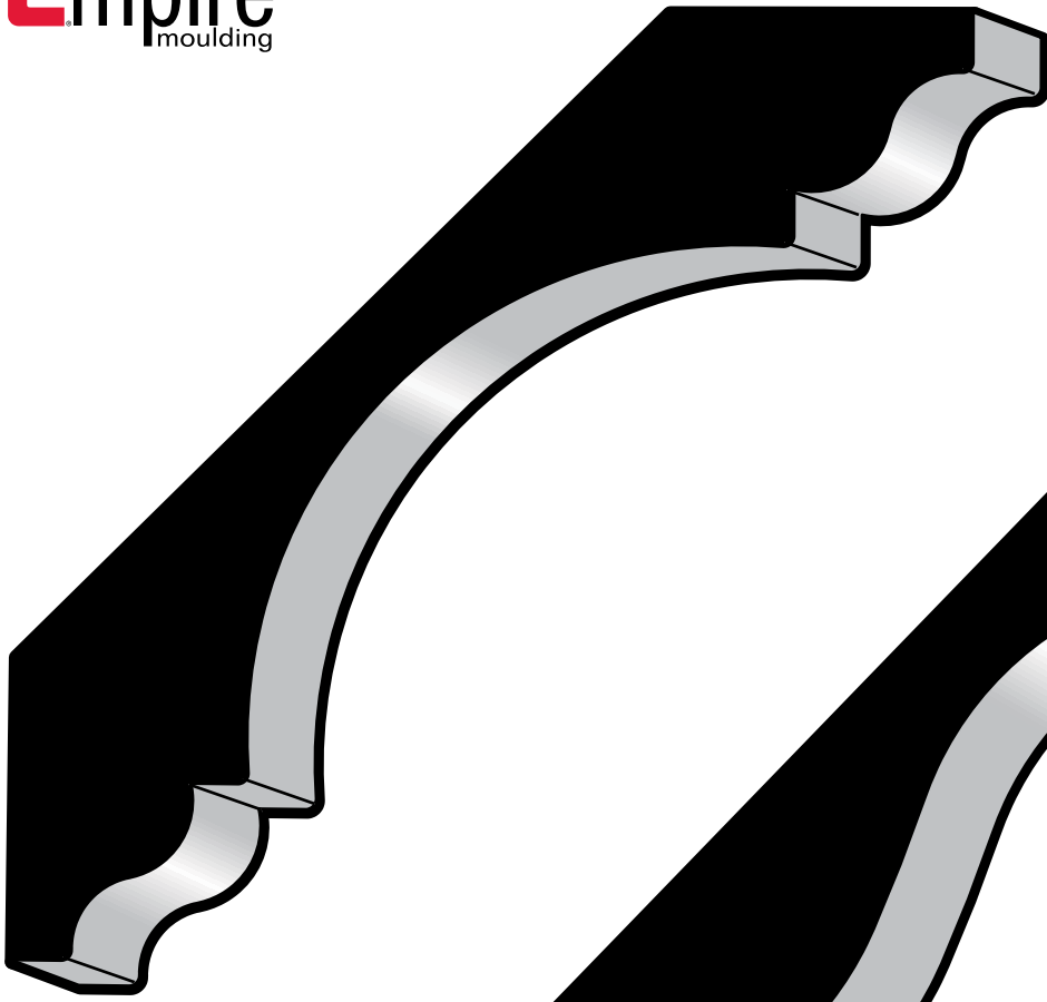
CROWN 041 1-3/16 x 6-5/16 MDF
