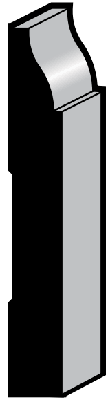
BASE L 634 7/16 x 3 3/8 x 2-3/4
